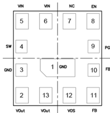
Figure 1-2 Pin Description
