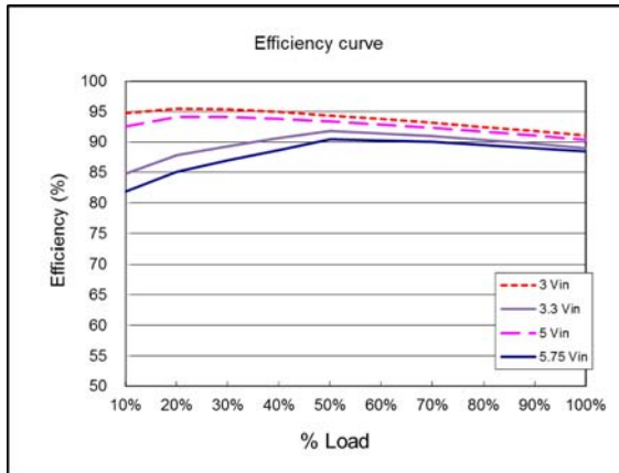
Efficiency curve ( V_{out} = 2.5\text{ V} )
