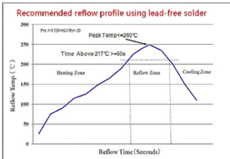
Figure 10-1 Recommended reflow profile using lead-free solder
