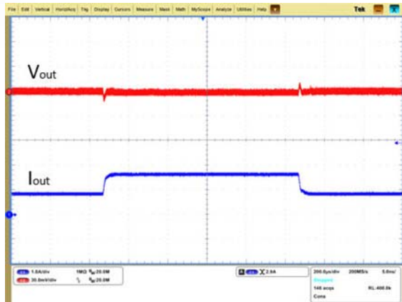
Load: 25% - 50% - 25%, di/dt = 5 A/ \mu s
