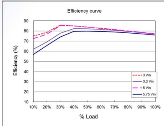
Efficiency curve ( V_{out} = 1.0\text{ V} )
