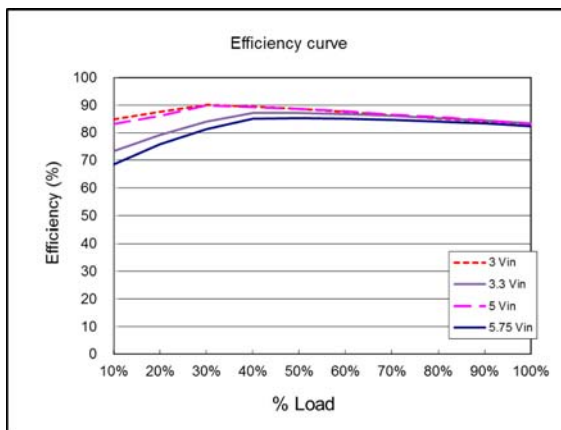
Efficiency curve ( V_{out} = 1.5\text{ V} )
