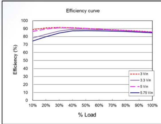
Efficiency curve ( V_{out} = 1.8\text{ V} )
