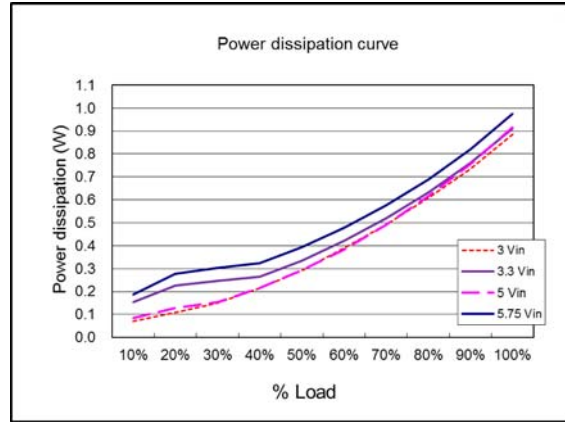
Power dissipation curve ( V_{out} = 1.8\text{ V} )
