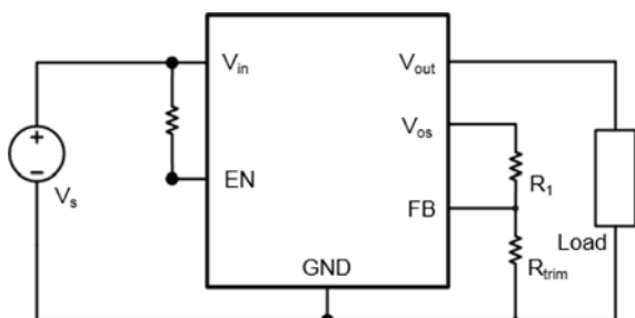
Figure 4-2 R_{trim} external connections
