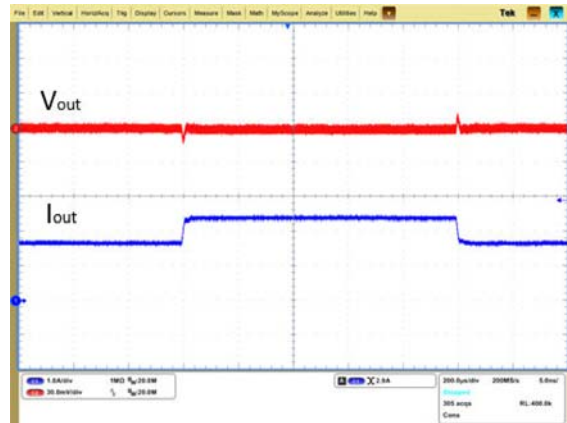
Load: 50% - 75% - 50%, di/dt = 5 A/ \mu s
