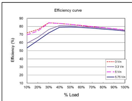
Efficiency curve ( V_{out} = 0.9\text{ V} )
