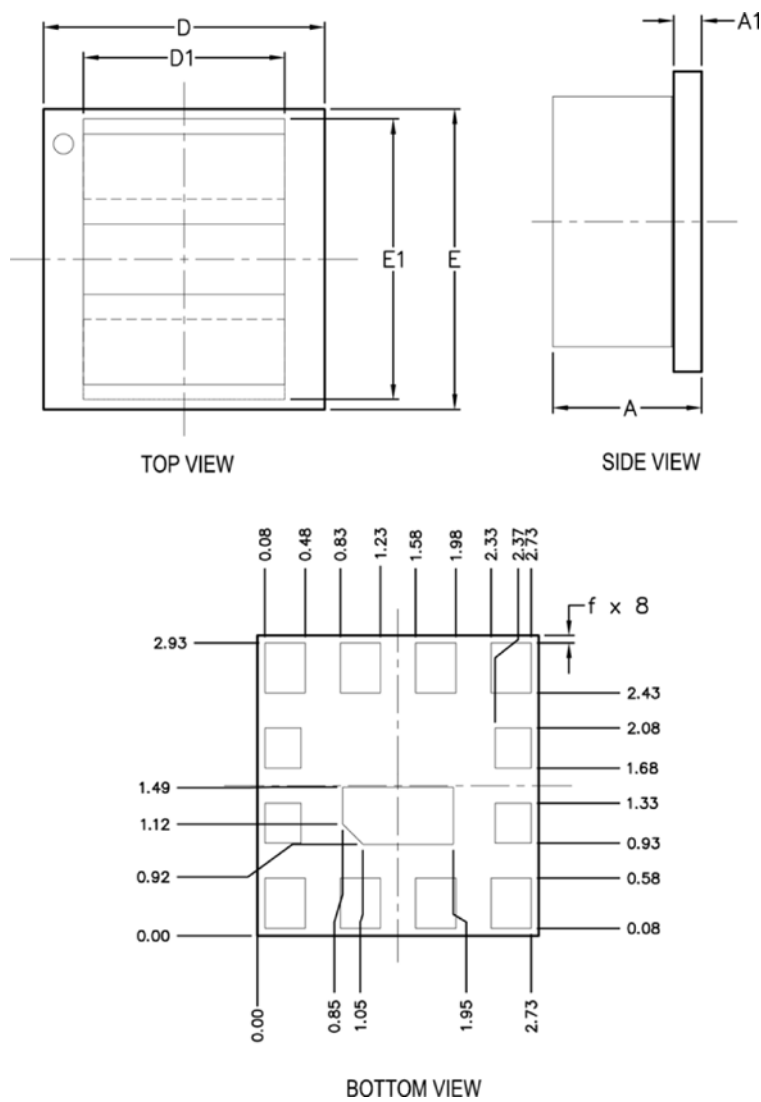
Figure 1-1 Mechanical diagram
