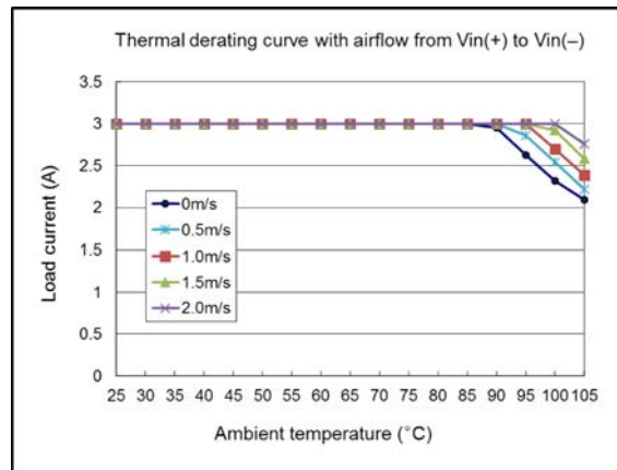
Thermal derating with airflow from V_{in}(+) to V_{in}(-) ( V_{in} = 3.3\text{ V} ; V_{out} = 1.8\text{ V} )
