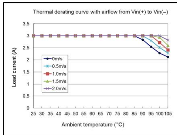
Thermal derating with airflow from V_{in}(+) to V_{in}(-) ( V_{in} = 5V ; V_{out} = 3.3V )
