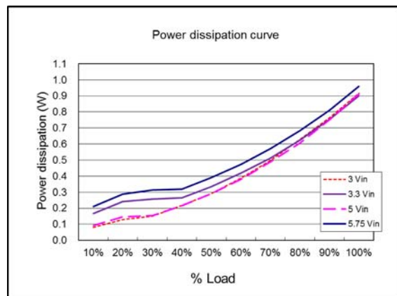
Power dissipation curve ( V_{out} = 1.5\text{ V} )
