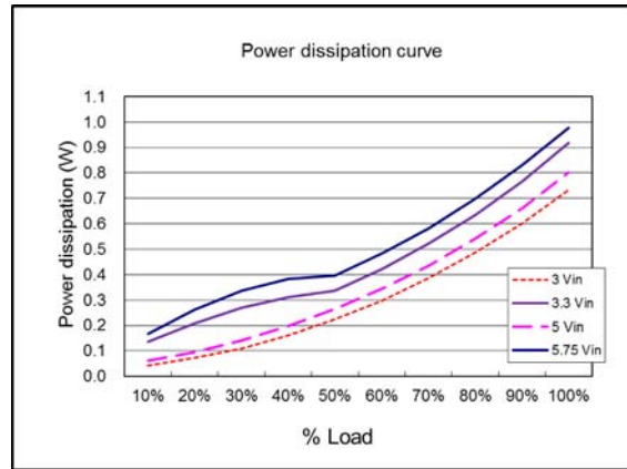
Power dissipation curve ( V_{out} = 2.5\text{ V} )
