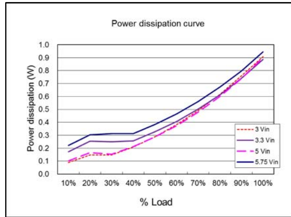
Power dissipation curve ( V_{out} = 1.2\text{ V} )
