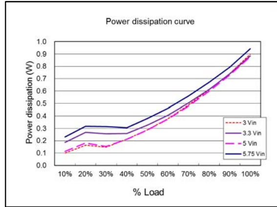
Power dissipation curve ( V_{out} = 1.0\text{ V} )
