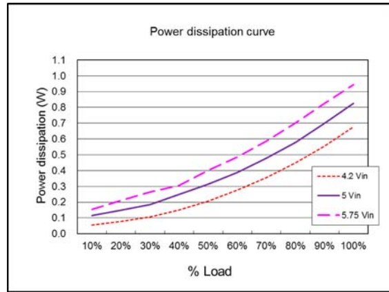
Power dissipation curve ( V_{out} = 3.7V )
