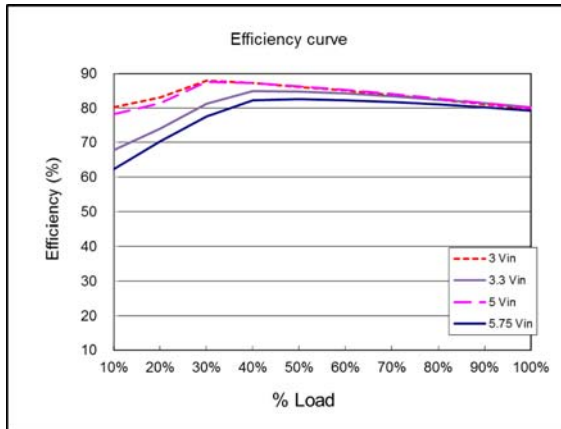
Efficiency curve ( V_{out} = 1.2\text{ V} )
