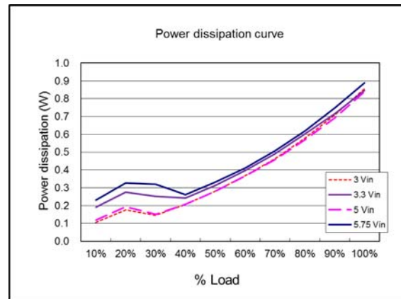
Power dissipation curve ( V_{out} = 0.8\text{ V} )
