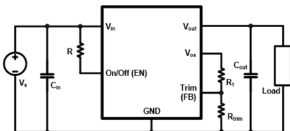
Figure 3-2 Application circuit
