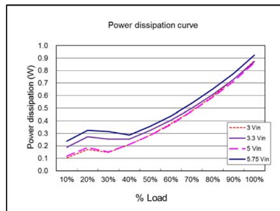
Power dissipation curve ( V_{out} = 0.9\text{ V} )
