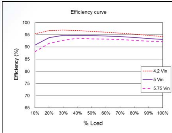
Efficiency curve ( V_{out} = 3.7V )
