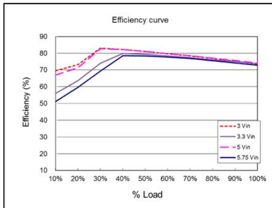
Efficiency curve ( V_{out} = 0.8\text{ V} )
