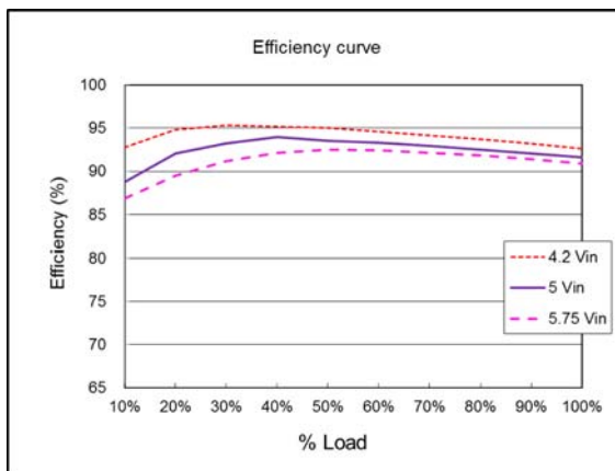
Efficiency curve ( V_{out} = 3.3\text{ V} )
