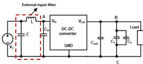
Figure 3-1 Test setup diagram
