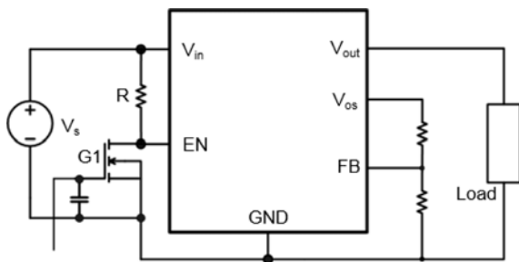
Figure 4-1 Circuit configuration for On/Off function
