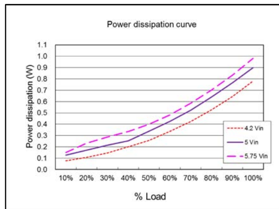
Power dissipation curve ( V_{out} = 3.3\text{ V} )
